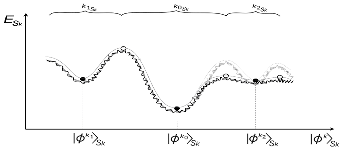
Figure 1. Schematic presentation of the adaptation of memory attractors in the energy-state space of the quantum-holographic Hopfield-like associative neural network of the biological macroscopic open quantum system S_k (local cellular ferment / substrate; local bodily acupuncture system / consciousness; non-local out-of-body consciousness / collective consciousness). This implies the necessity of quantum-informational successive bioresonance balancing of all unwanted lateral memory attractors (as in the picture), which would otherwise cause the development of psychosomatic diseases at the individual level and interpersonal conflicts in this and future generations at the collective level – with hints for reorientation to ecologically holistic subtle actions for solutions of the global risk society [15,16].
