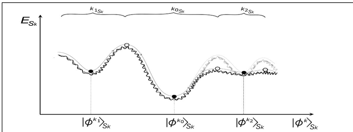
Figure 2. Schematic presentation of the adaptation of memory attractors in the energy-state hypersurface of the quantum-holographic memory / propagator of various hierarchical levels of biological macroscopic open quantum system(s) S_k [6] (local cell's biomolecular protein / target, local acupuncture system / consciousness, or nonlocal out-of-body consciousness / collective consciousness). This implies necessity of quantum-informational successive bioresonant removing of all unwilling side memory attractors (like \phi^{k_2} in Figure 2), which would otherwise cause development of psychosomatic diseases on the individual level, and interpersonal fights in this and further generations on the collective level.
