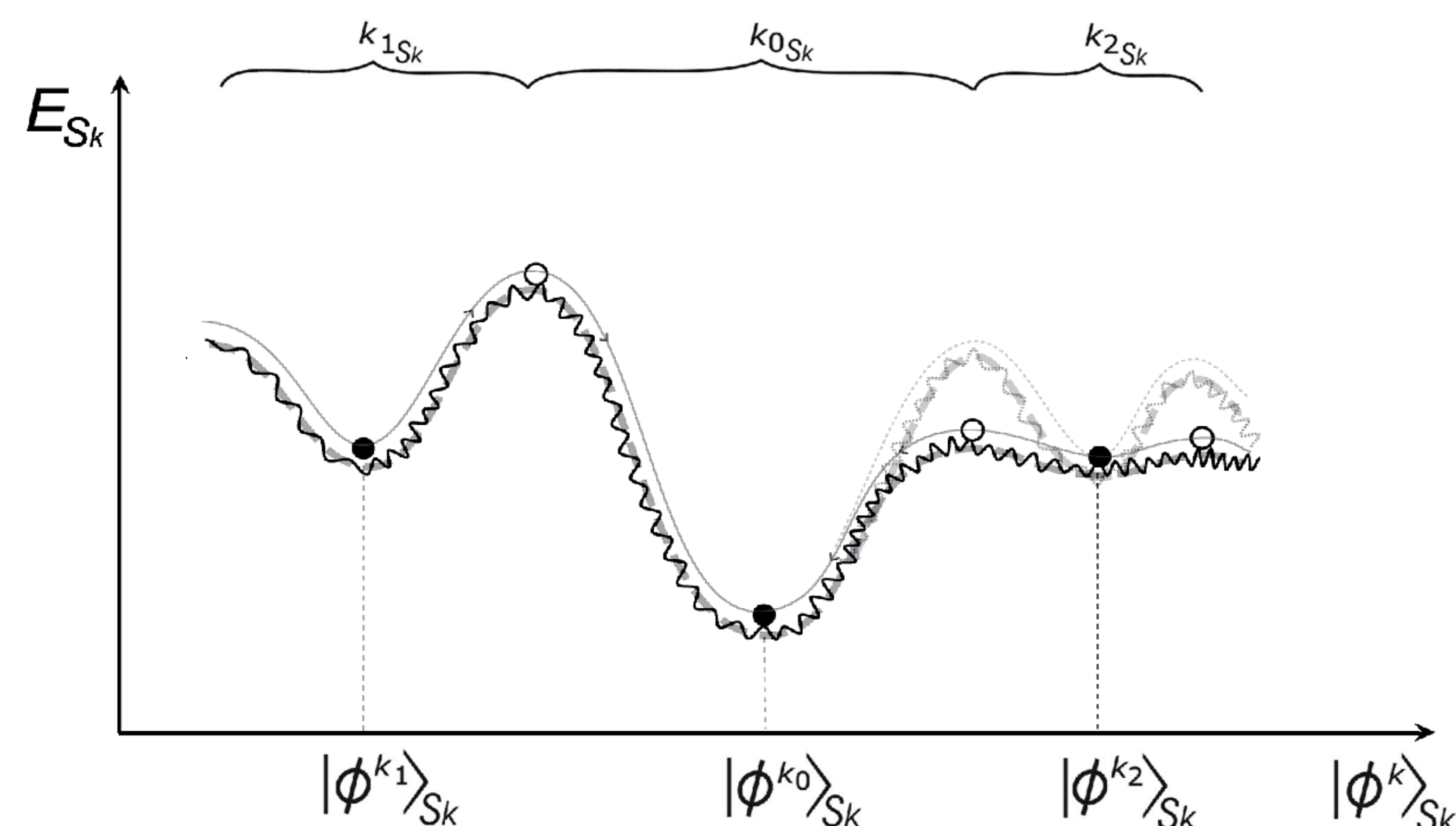
Figure 1. Schematic presentation of the memory attractors in the energy-state hypersurface of psychosomatic state of open macroscopic quantum-holographic acupuncture system / consciousness, as proposed quantum-holographic manifestations of psychosomatic disorders (hundreds of them being in primary psychosomatic diseases and thousands of them in their combinations according to acupuncture-based Tibetan traditional medicine, with therapeutic goal to balance / remove all unwilling side memory attractors in procedure traditionally recommended half a year). Then, in the context of holistic acupuncture-based and consciousness-based approaches and techniques [7], their goal would be bioresonant excitation of the target palpatory-painful / psychologically-traumatic memory attractors of acupuncture system / consciousness. That enables disordered initial memory attractors to be one by one resonantly excited (similar to annealing procedure in artificial neural networks [9]), thus becoming shallower and wider on the account of deepening of (energy-dominating) memory attractor of the healthy quantum state (acupuncture palpatory painless / psychologically non-traumatic). This information of the healthy quantum state is then altogether quantum-holographically projected on lower quantum-holographic cellular level, thus changing the expression of genes in morphogenesis. Therefore, all holistic acupuncture-based & consciousness-based approaches and techniques could be treated as quantum-informational therapies, by imposing new healing boundary conditions in the energy-state space of the acupuncture system / consciousness.
