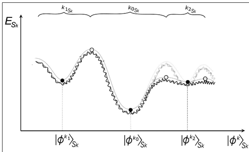
Figure 1. Schematic presentation of the adaptation of memory attractors in the energy-state E_{S_k}(\phi^k) hypersurface of the quantum-holographic memory of various hierarchical levels of biological macroscopic open quantum systems S_k [3-8] (local cell's protein-target biomolecular one, local acupuncture system/ consciousness, or nonlocal out-of-body consciousness/collective consciousness):
