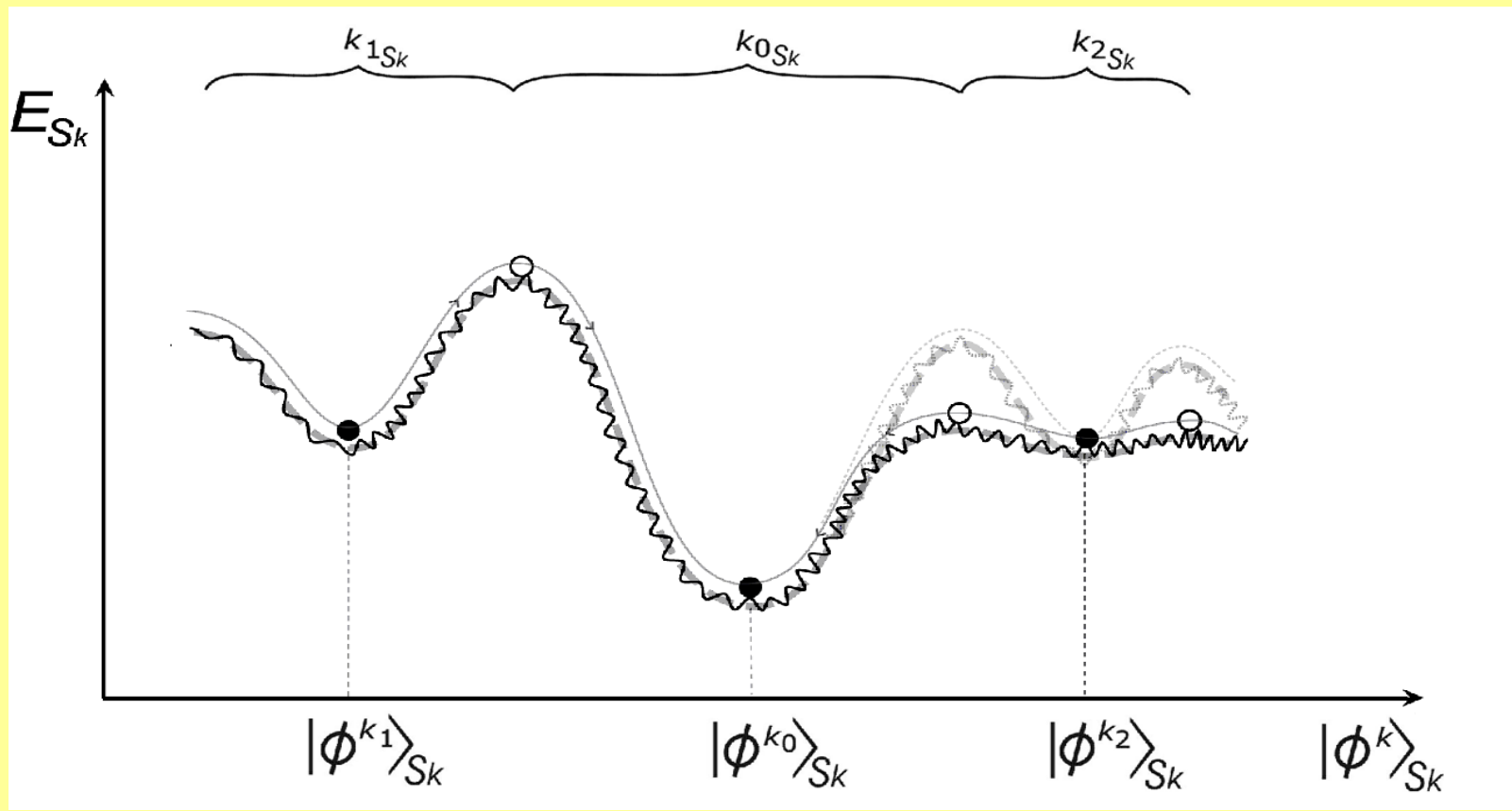
Figure 3. Schematic presentation of adaptation of memory attractors in energy-configuration hypersurface of quantum-holographic memory / propagator of various hierarchical levels of biological macroscopic open quantum system(s) S_k [2] ( local cell's biomolecular protein / target, local acupuncture system / consciousness, or nonlocal out-of-body consciousness / Collective consciousness ). This implies necessity of quantum-informational successive bioresonant balansing of all unwilling side memory attractors (like \phi^{k_2} in the figure), which would otherwise cause development of psychosomatic diseases on individual level & interpersonal fights in this & further generations on collective level.
