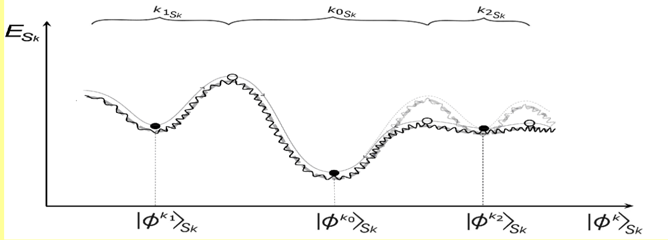
Figure 2. Schematic presentation of the adaptation of memory attractors in the energy-state ( E_{S_k}(\phi^k) ) hypersurface of the quantum-holographic memory of various hierarchical levels of biological macroscopic open quantum systems S_k ( local cell's biomolecular protein-target, local acupuncture system-consciousness, or nonlocal out-of-body consciousness-collective consciousness ) [6]:
