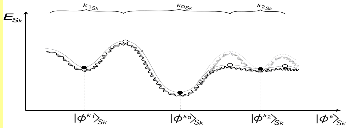
Fig. 1. Schematic presentation of the memory attractors in the energy-state hypersurface of psychosomatic state of open macroscopic quantum-holographic acupuncture system/consciousness , as proposed quantum-holographic manifestations of psychosomatic disorders (hundreds of them being in primary psychosomatic diseases and thousands of them in their combinations according to acupuncture-based Tibetan traditional medicine , with therapeutic goal to balance / remove all unwilling side memory attractors in procedure traditionally recommended half a year). Then, in the context of holistic acupuncture-based and consciousness-based approaches and techniques [7], their goal would be bioresonant excitation of the target palpatory-painful/psychologically-traumatic memory attractors of acupuncture system/consciousness. That enables disordered initial memory attractors to be one by one resonantly excited (similar to annealing procedure in artificial neural networks [9]), thus becoming shallower and wider on the account of deepening of (energy-dominating) memory attractor of the healthy quantum state (acupuncture palpatory painless/psychologically non-traumatic). This information of the healthy quantum state is then altogether quantum-holographically projected on lower quantum-holographic cellular level, thus changing the expression of genes in morphogenesis . Therefore, all holistic acupuncture-based & consciousness-based approaches and techniques could be treated as quantum-informational therapies , by imposing new healing boundary conditions in the energy-state space of the acupuncture system/consciousness.
