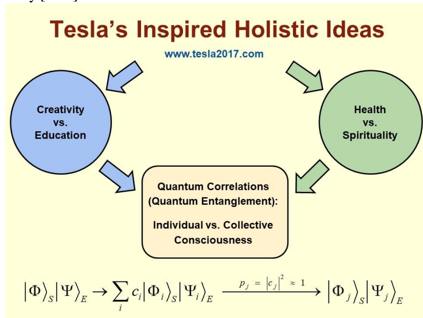
Figure 1. (a) Symbolic representation of mentally controlled-directed increasing of macro-quantum correlations of interacting individual consciousness ( S ) and collective consciousness / environment ( E ) in transpersonally-entangling creative phases (left-hand side of the image and formula above, with previous mental increase of the focused weight contribution c_j and subsequent (practically non-stochastic) classically-reduced selection of this dominant weight contribution c_j ); and (b) Symbolic representation of mentally controlled-systemic decreasing of macro-quantum correlations of interacting individual consciousness ( S ) and collective consciousness / environment ( E ) in transpersonally-disentangling spiritual phases (right-hand side of the image and formula above, with previously systemic mental decreasing of almost all weight contributions c_i and subsequent (practically non-stochastic) classically-reduced selection of the remaining dominant weight contribution c_j (related to mentally-embedded address on the founder of the corresponding mystical tradition)).
