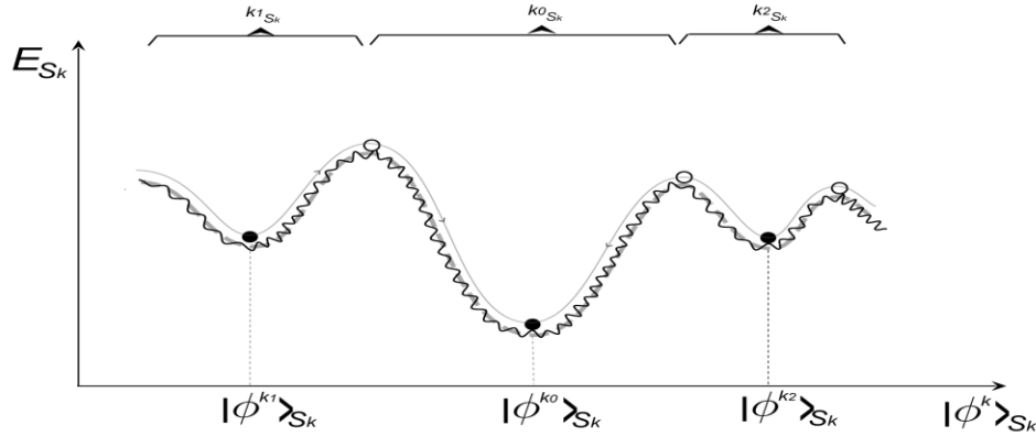
Figure 2. Schematic presentation of the memory attractors in the energy-state hypersurface of psychosomatic state of open macroscopic quantum-holographic acupuncture system / consciousness , as proposed quantum-holographic manifestations of psychosomatic disorders (hundreds of them being in primary psychosomatic diseases and thousands of them in their combinations according to acupuncture-based Tibetan traditional medicine , with therapeutic goal to balance / remove all unwilling side memory attractors in procedure traditionally recommended half a year) [2-6]. This information might be quantum-holographically projected onto lower open macroscopic quantum-holographic cellular enzyme-gene level (which also functions on quantum-holographic-like cellular quantum-conformational level of the molecular recognition, thus influencing gene expression & possible somatisation of the top-down hierarchically projected non-balanced / non-removed psychosomatic disordered information). On the other hand, higher open macroscopic hierarchical level of quantum-holographic collective consciousness & related (quantum) holistic global psychosomatics might also be quantum-holographically projected onto lower levels of quantum-holographic individual acupuncture systems / consciousnesses (with spiritual / social implications on the necessity of transpersonal quantum-holographic removing of all unwilling side memory attractors on the level of collective consciousness, which unless would result in further transpersonal transfer of memory attractors onto individual & collective consciousnesses in this and future generations). See the text for further explanation.
