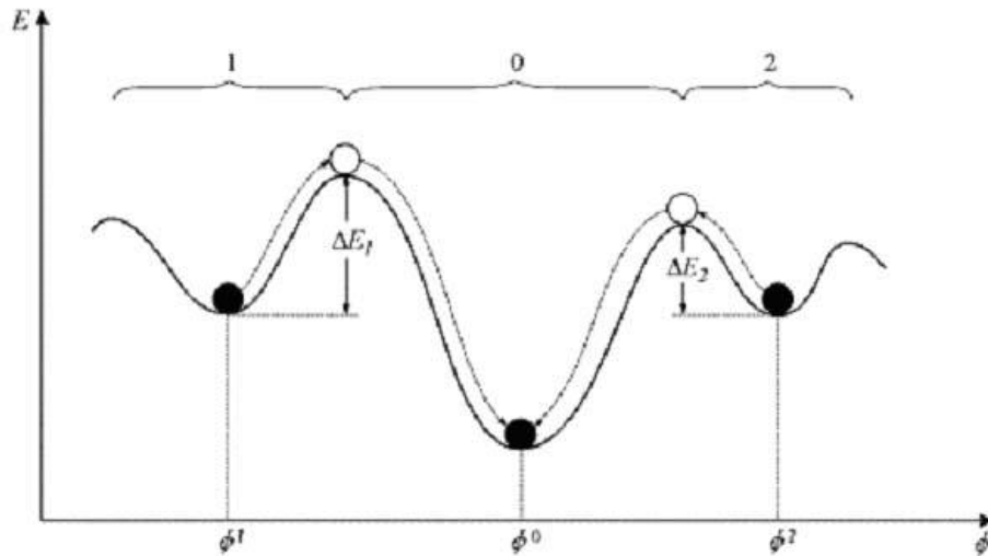
Fig. 1. Schematic presentation of the potential hypersurface of nonlocal selfconsistent macroscopic quantum potential in the acupuncture energy-state space ( E, \phi ): 0 - basin of attraction of the ground (healthy) state \phi^0 ; 1 and 2 - basins of attraction of the two excited (psychosomatically disordered) states \phi^1 and \phi^2 (hundreds of them being in general). It should be pointed out that energy surface changes gradually during the MRT treatment, by decreasing the potential barriers \Delta E_1 and \Delta E_2 (and corresponding MRT sensory responses) of the potential wells 1 or 2, to be overcome in traversing to the 0 basin of attraction of the ground (healthy) state, when organism gradually recovers by further spontaneous approaching the healthy state \phi^0 (with poor MRT sensory response, as already being in the ground-state). Such a picture is very close to the associative neural networks ones in their energy-configuration spaces, and to pattern recognition as convergence of the neural networks to the bottoms of the potential hypersurfaces, being the attractors of neural networks memory patterns \phi^0, \phi^1, \phi^2 .
